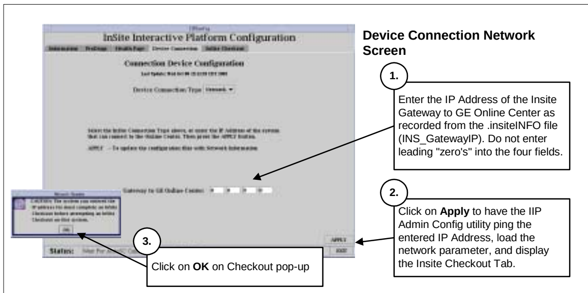
Figure 6 Insite Interactive Platform Configuration Device Connection Tab – Network Setup
